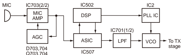
Fig. 4 Transmitter System
