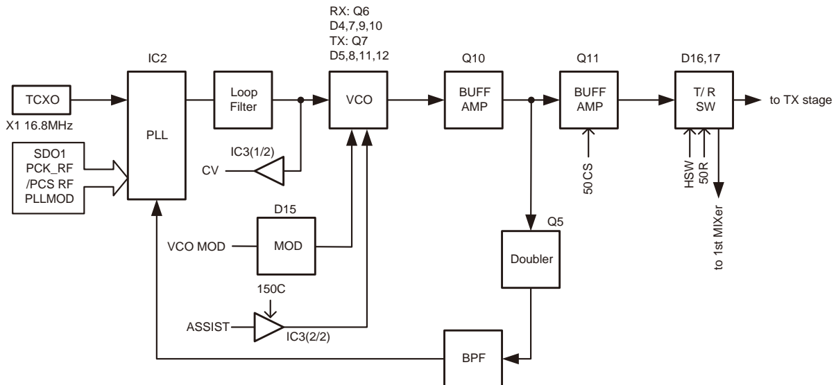
Fig. 6 PLL circuit
